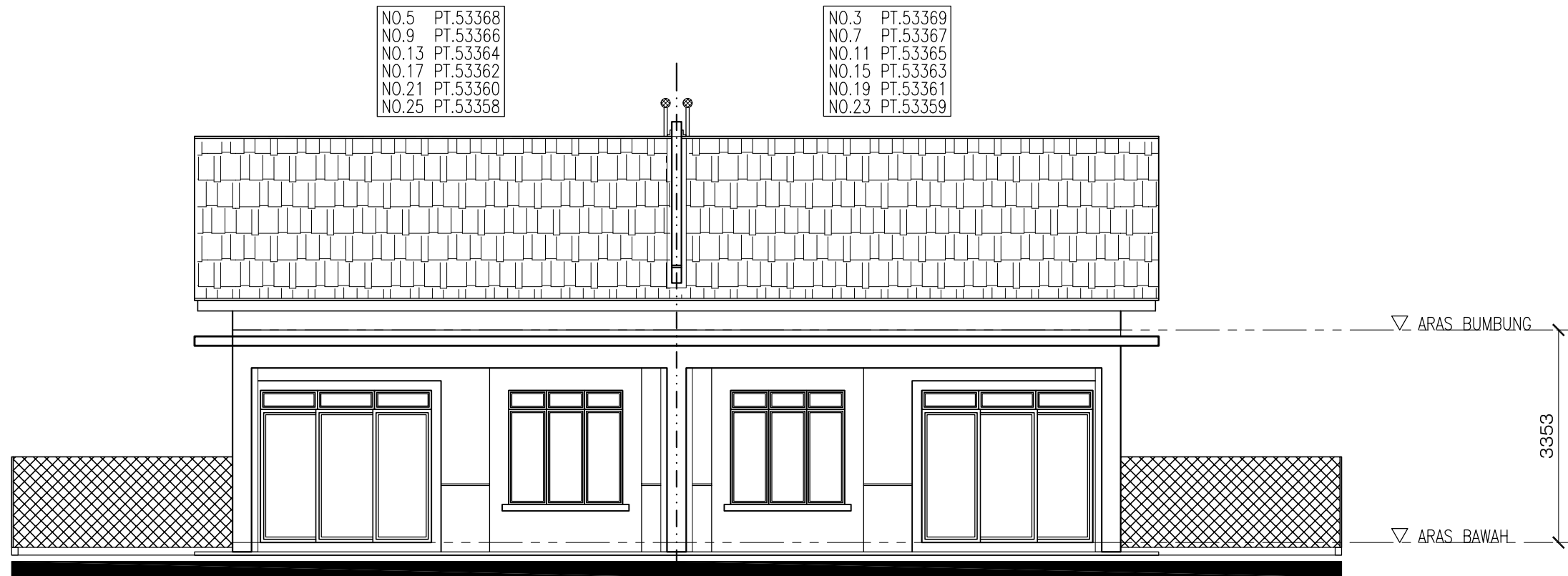
PANDANGAN HADAPAN
