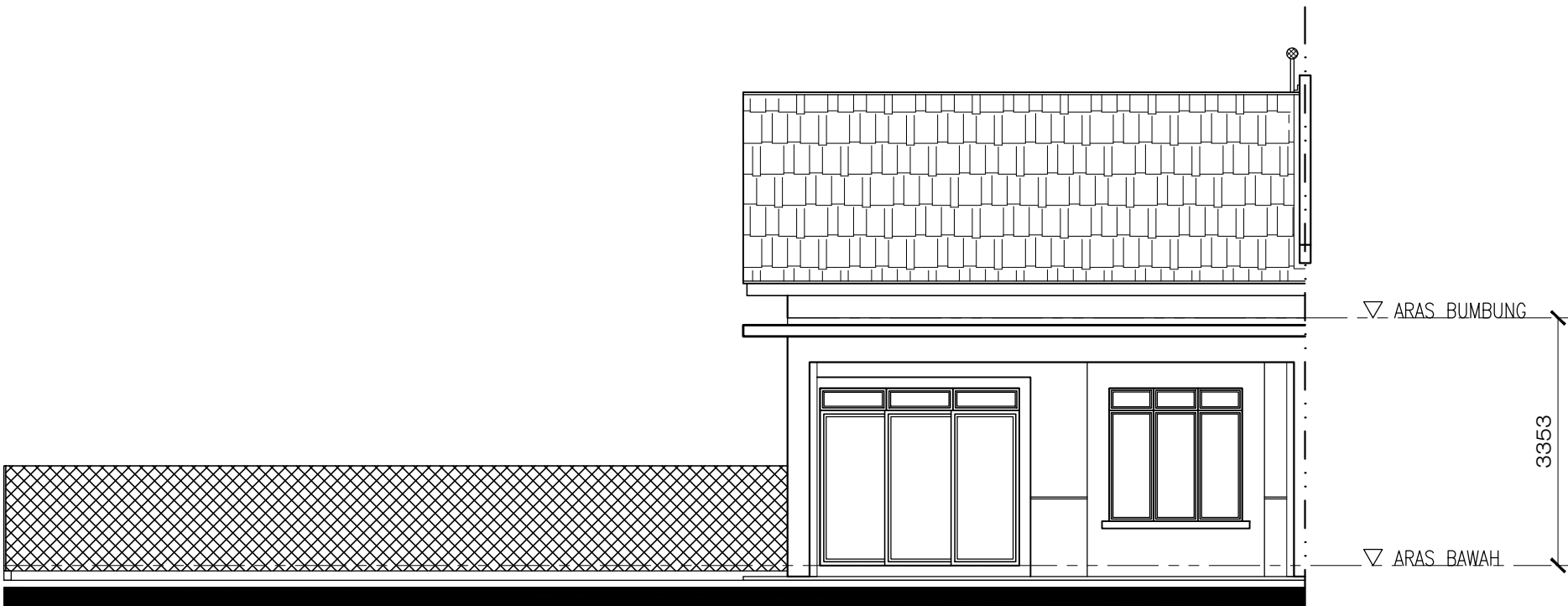
PANDANGAN HADAPAN
